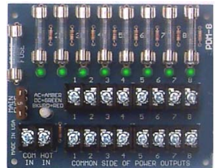
Optional Accessories Fig: PDM-8 Power Distribution Module
