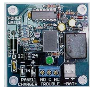
Fig: PW-1 Battery Supervision Module for LP-3
